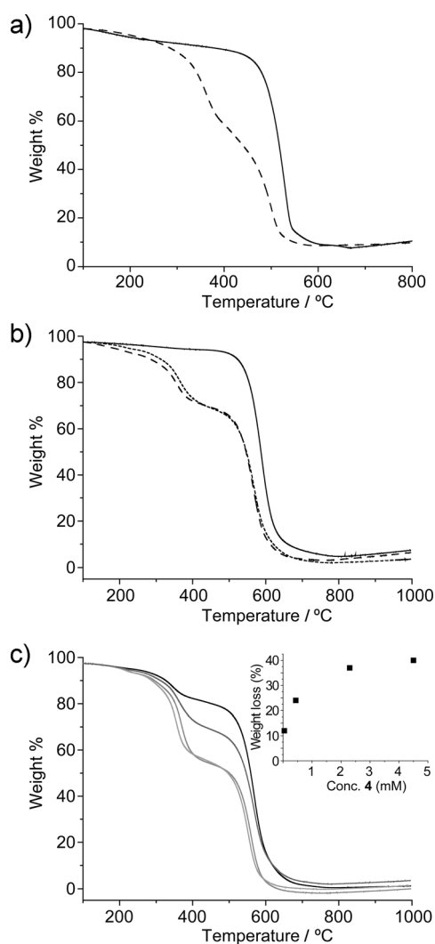
Figure 2. a) TGA analysis (air, 10^{\circ}\text{C min}^{-1} ) of pristine (7,6)-enriched SWNTs (solid line) and the product formed by treatment with 4 (10 mg, 0.0087 mmol) and the Grubbs second-generation catalyst in TCE (20 mL) at room temperature for 72 h (dashed line). b) TGA analysis (air, 10^{\circ}\text{C min}^{-1} ) of pristine plasma-purified SWNTs (solid line), the product formed by treatment with 4 (10 mg, 0.0087 mmol) and the Grubbs second-generation catalyst in TCE (20 mL) at room temperature for 72 h (dotted line), and the same sample after heating at reflux in TCE for 30 min and filtration (dashed line, showing the stability of the noncovalent modification). c) Variation in the degree of functionalization with the relative concentration of 4 with respect to that of the SWNTs, as shown by TGA analysis (air, 10^{\circ}\text{C min}^{-1} ): 0.044 mM (black), 0.44 mM (dark gray), 2.3 mM (gray), and 4.5 mM (light gray). Inset shows the relative weight loss versus the concentration of 4 .
